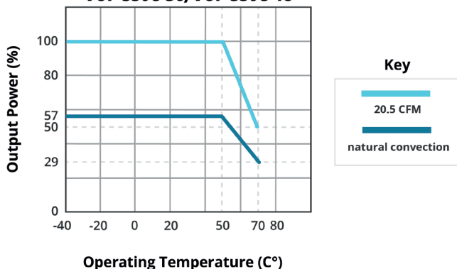
TEMPERATURE DERATING CURVE (full load 350W with 20.5 CFM) VOF-350C-24, VOF-350C-27 VOF-350C-36, VOF-350C-48
