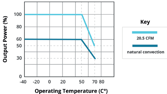
TEMPERATURE DERATING CURVE (full load 300W with 20.5 CFM) VOF-350C-12
