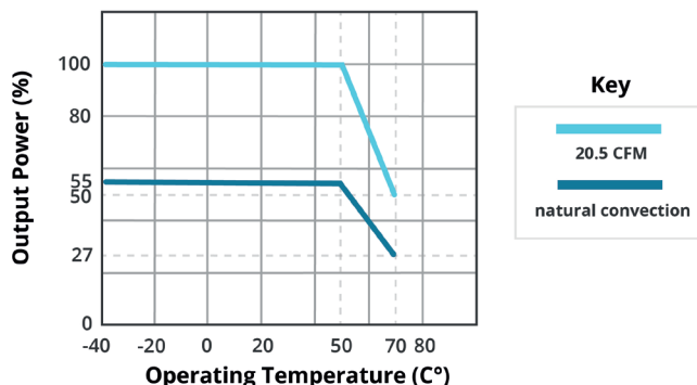
TEMPERATURE DERATING CURVE (full load 325W with 20.5 CFM) VOF-350C-15
